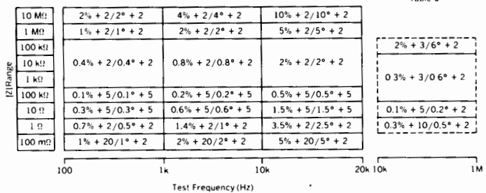
HP 4276A Measurement Range HP 4277A Measurement Range
