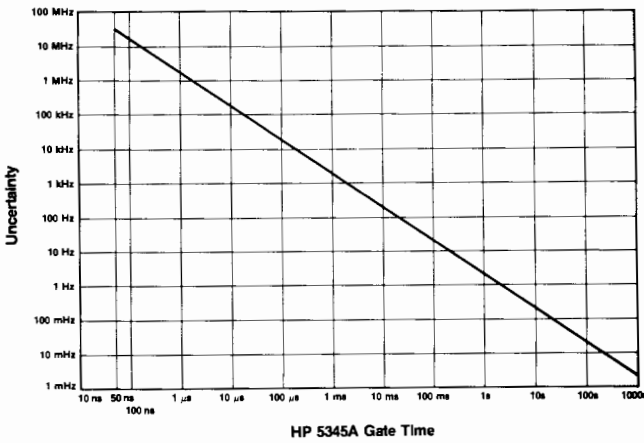
Graph 1. Uncertainty ( 2 \times \text{LSD} ) due to selected 5345A gate time.
