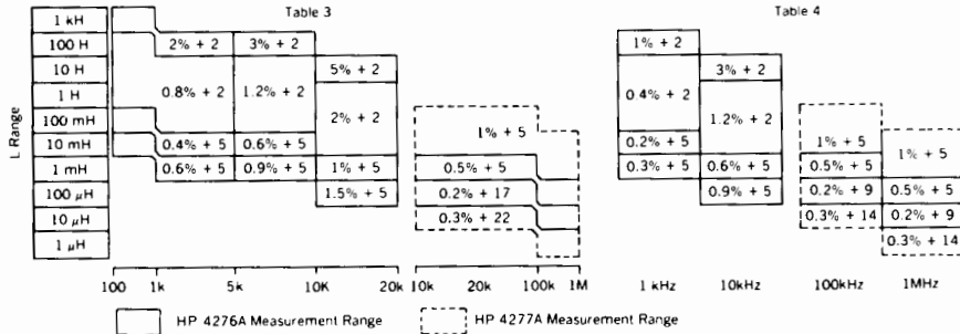
HP 4276A Measurement Range HP 4277A Measurement Range
